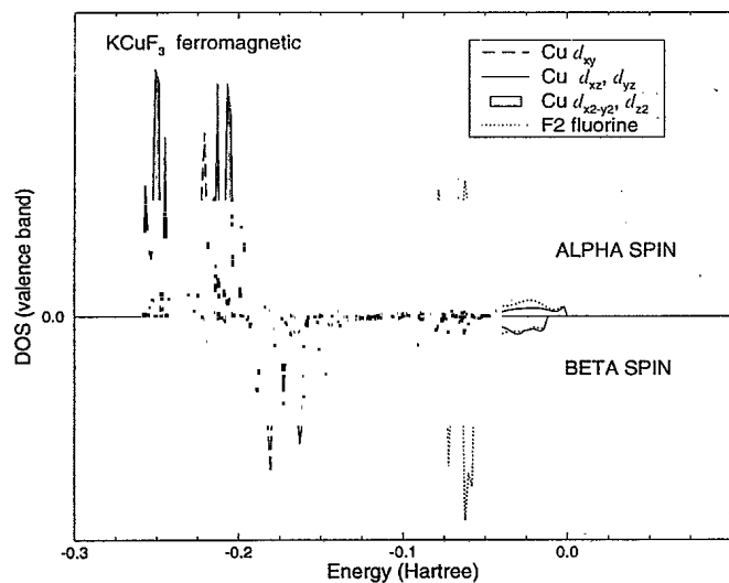
FIG. 4. Valence-band projected density of states for ferromagnetic phase of \text{KCuF}_3 . Energy relative to the highest occupied level.
