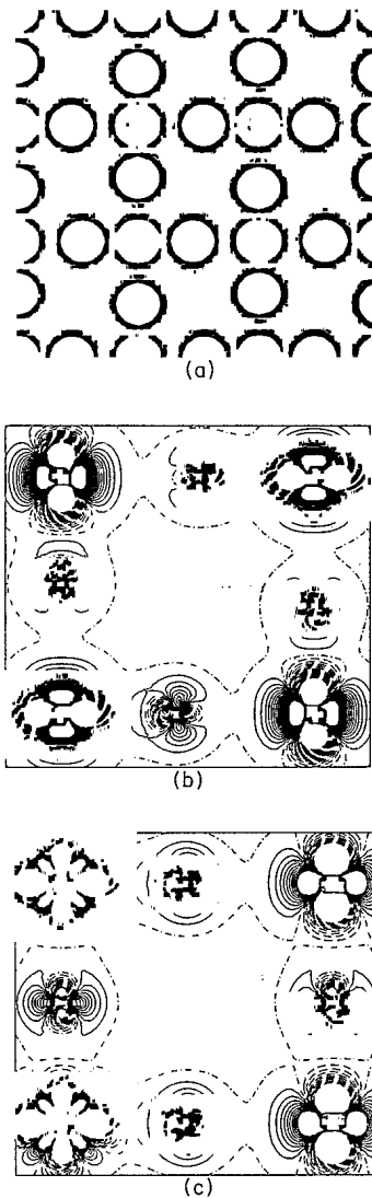
FIG. 3. (a) Total charge-density map in the ab (001) plane of \text{KCuF}_3 through the Cu and F ions. The separation between adjacent isodensity curves is 0.01 e/\text{bohr}^3 ; the innermost curves in the atomic region correspond to 0.15 e/\text{bohr}^3 . The dashed box denotes the area of (b), which is a charge density difference map in the ab plane for AF1 \text{KCuF}_3 . (c) is the equivalent plot in the ac plane. Both (b) and (c) refer to the difference between the bulk density and the density obtained as a superposition of spherical ionic densities (using the same basis set in both cases). Continuous, dashed and dot-dashed lines correspond to positive, negative, and zero values, respectively. The separation between adjacent isodensity curves is 0.005 e/\text{bohr}^3 ; the innermost curves in the atomic region correspond to 0.05 e/\text{bohr}^3 .
