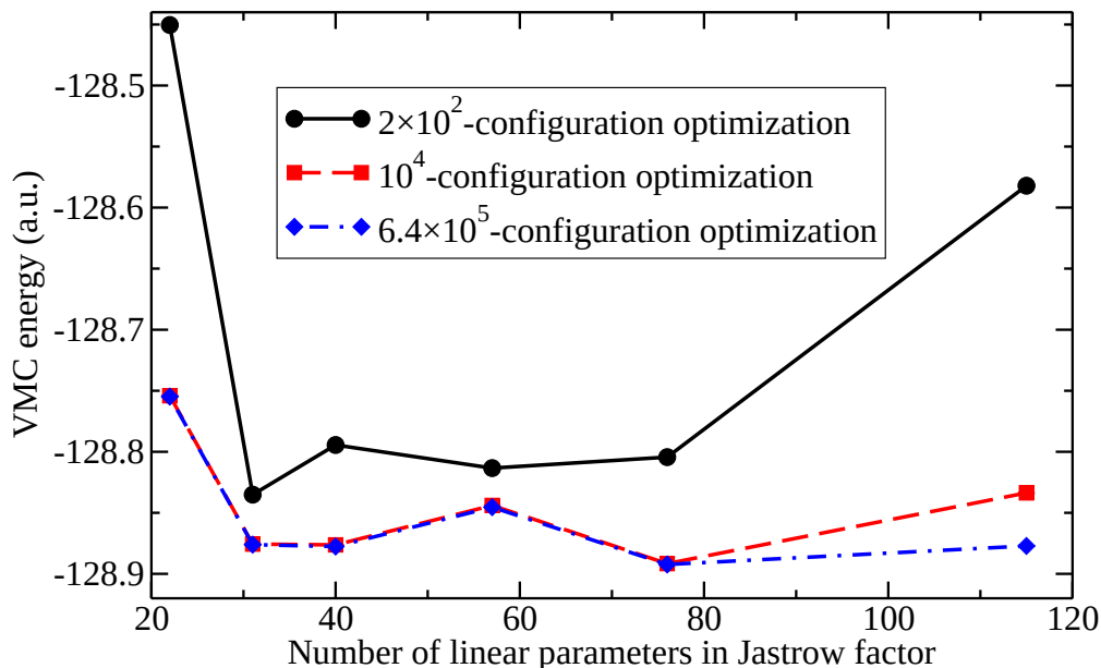
FIG. 12: (Color online) The VMC energy of an all-electron neon atom against the number of parameters in the Jastrow factor. Different numbers of configurations were used to carry out the unweighted variance-minimization calculations. Six optimization cycles were performed in order to guarantee self-consistency. Very long VMC simulations were carried out using the optimized Jastrow factors in order to obtain the energies plotted in the graph. The VMC error bars are smaller than the symbols. The Slater wave function contained Hartree-Fock orbitals.
