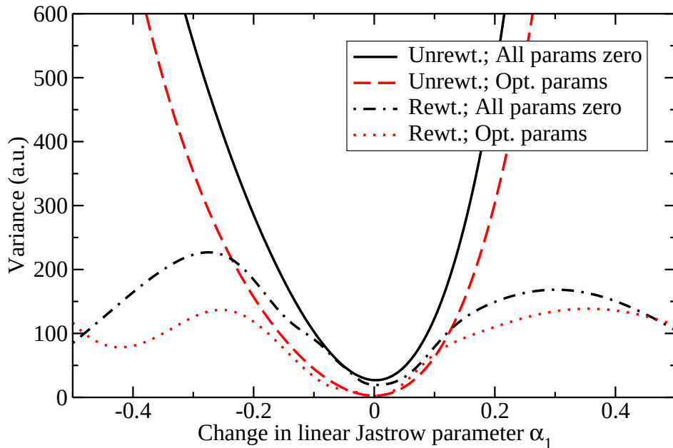
FIG. 5: (Color online) The reweighted and unweighted variance for an all-electron neon atom plotted against the change in the value of a linear Jastrow parameter, \alpha_1 . Plots are shown for the case in which all the parameters are set to zero and the case in which all the parameters have been optimized. The set of 100 configurations used to calculate the variance were distributed according to the square of the Hartree-Fock wave function. The Jastrow factor contained a total of 27 linear parameters.
