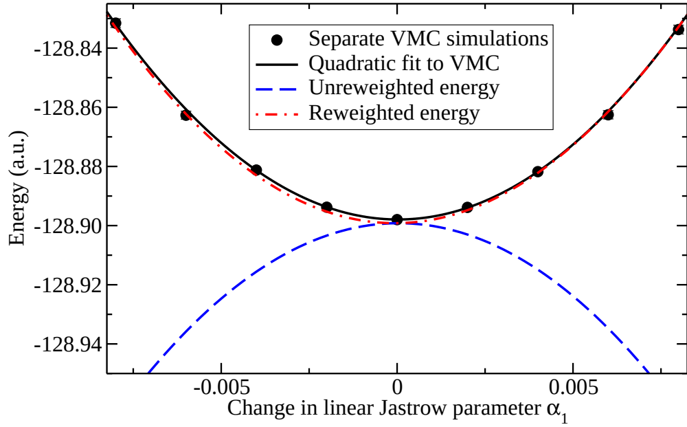
FIG. 8: (Color online) The VMC energy of an all-electron neon atom against the change in the value of a linear Jastrow parameter \alpha_1 from the value determined by self-consistent unweighted variance minimization. Specifically, the Jastrow factor was the best all-electron neon Jastrow factor described in Ref. 5 . The reweighted and unweighted energies calculated using 8 \times 10^5 configurations distributed according to the square of the optimized wave function are also plotted. The statistical error bars in the VMC data are smaller than the symbols.
