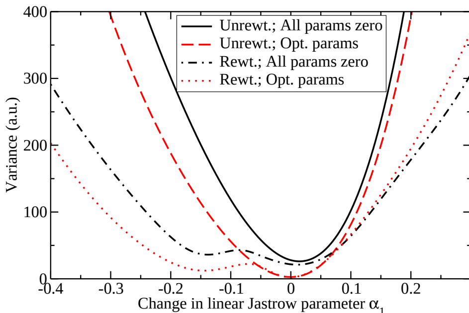
FIG. 6: (Color online) The same as Figure 5 except that 10^4 configurations were used to calculate the variance.
