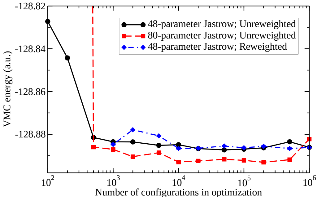
FIG. 10: (Color online) The VMC energy of an all-electron neon atom against the number of configurations used to optimize the linear Jastrow parameters in an unweighted variance minimization. Eight optimization cycles were performed for each number of configurations in order to ensure that self-consistency was achieved. The Slater wave function contained Hartree-Fock orbitals. The error bars in the VMC data are smaller than the symbols.
