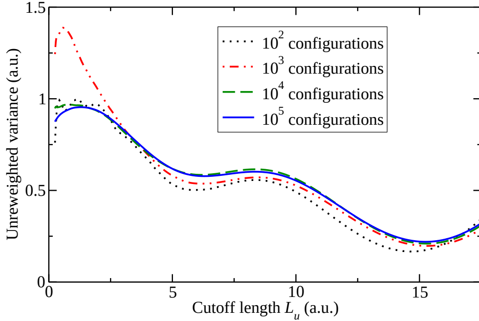
FIG. 3: (Color online) The unweighted variance \sigma_u^2 for an \text{SiH}_4 molecule (with a Hartree-Fock silicon pseudopotential 7 ) plotted against the cutoff length for the electron-electron terms in the Jastrow factor, L_u . The Jastrow factor is such that the local energy is continuous when an electron-electron separation passes through the cutoff length. 5 Different numbers of VMC-generated configurations were used to calculate the unweighted variance. All of the linear Jastrow parameters are set to zero. In each case the configurations were distributed according to the square of the Hartree-Fock wave function. The Jastrow factor contained a total of 56 linear parameters, plus three cutoff lengths.
