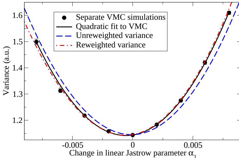
FIG. 9: (Color online) The same as Fig. 8 except that the VMC variance is plotted against the change in the parameter value.
