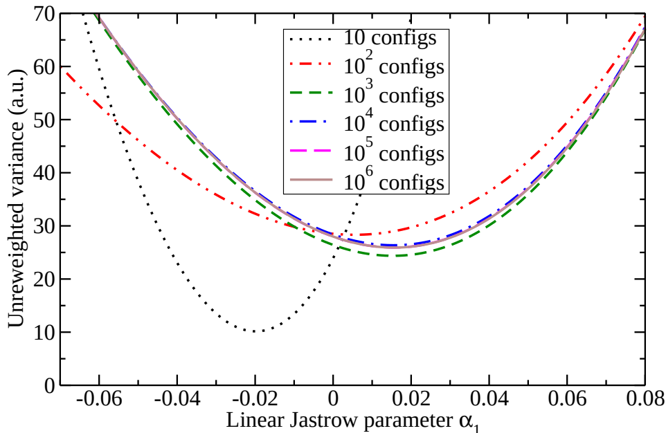
FIG. 1: (Color online) The unweighted variance \sigma_u^2 for an all-electron neon atom plotted against one of the linear Jastrow parameters. All of the other linear parameters are set to zero. Different numbers of configurations were used to calculate the quartic coefficients of the unweighted variance. In each case the configurations were distributed according to the square of the Hartree-Fock wave function. The Jastrow factor contained a total of 24 linear parameters. The curves for 10^5 and 10^6 configurations are indistinguishable in the figure.
