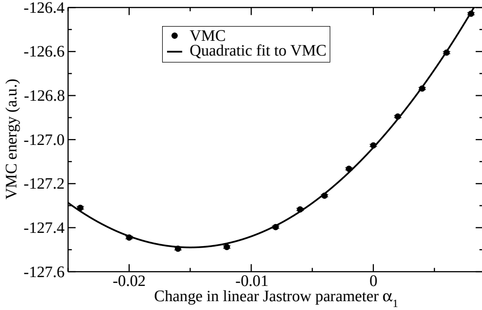
FIG. 7: The VMC energy of an all-electron neon atom against the change in the value of a linear Jastrow parameter \alpha_1 from the value determined by self-consistent unweighted variance minimization. The Jastrow factor was chosen to be poor, with no electron-nucleus or electron-electron-nucleus terms, and the same electron-electron terms were used for both parallel and antiparallel spins. There is only one optimizable parameter: \alpha_1 .
