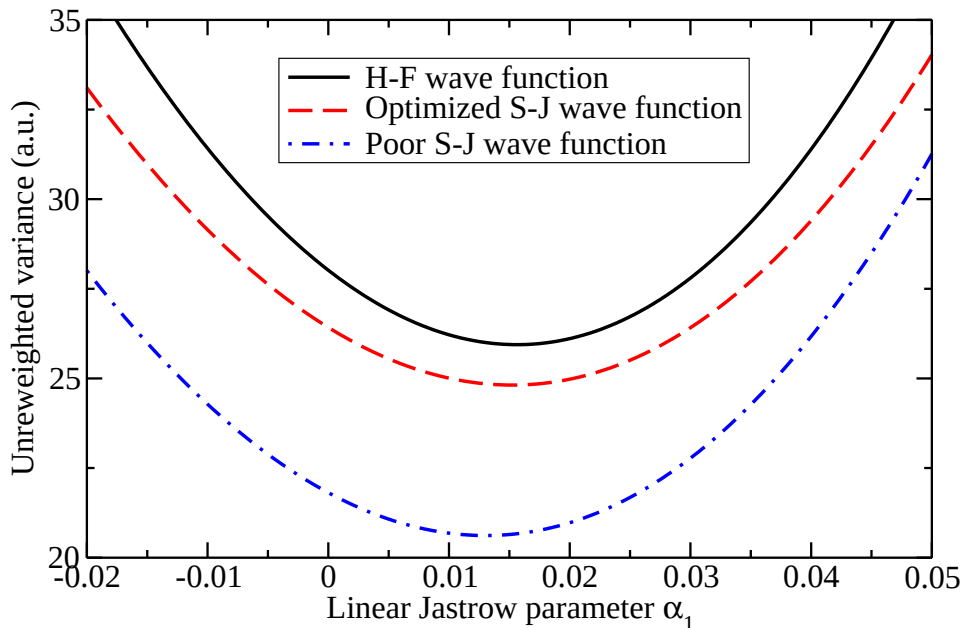
FIG. 11: (Color online) The unweighted variance for an all-electron neon atom plotted against the value of the linear Jastrow parameter \alpha_1 for three different configuration distributions: the square of the Hartree-Fock wave function, the square of an optimized Slater-Jastrow wave function and the square of a poor Slater-Jastrow wave function. 10^6 configurations were used to calculate the unweighted variance. The Jastrow factor contained a total of 36 linear parameters. The Slater wave function contained Hartree-Fock orbitals.
