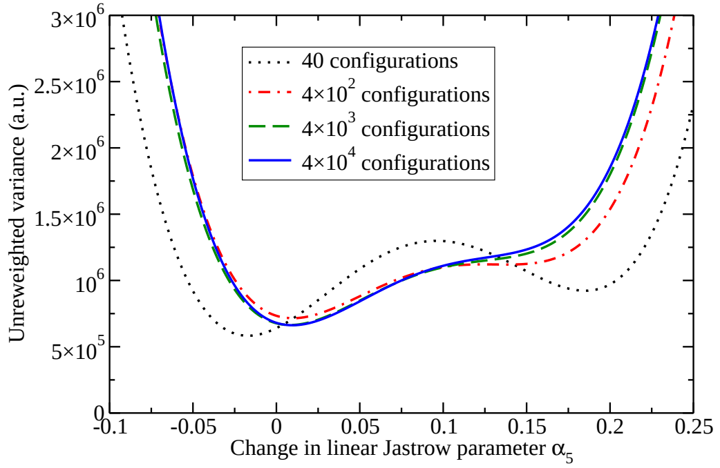
FIG. 2: (Color online) The unweighted variance \sigma_u^2 for an all-electron neon atom plotted against the change in one of the linear Jastrow parameters. All the parameters in the Jastrow factor are set to large, random values. Different numbers of VMC-generated configurations were used to calculate the quartic coefficients of the unweighted variance. In each case the configurations were distributed according to the square of a Slater-Jastrow wave function, where the Jastrow factor contained the random parameters, so that the resulting distribution was very unlike the ground-state distribution. The Jastrow factor contained a total of 72 linear parameters. The Slater wave function contained Hartree-Fock orbitals.
